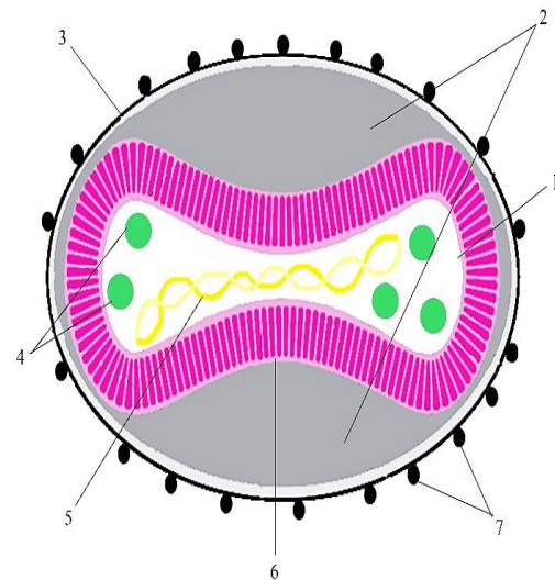
Fig. 1: A poxvirus particle.
