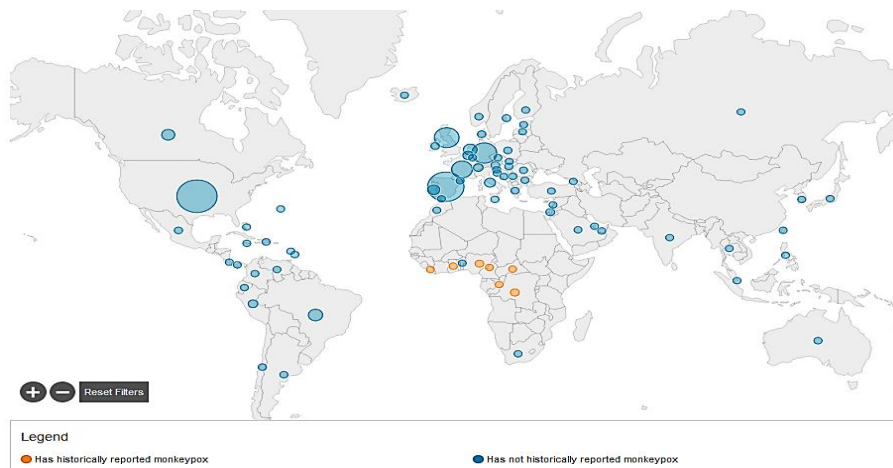
Fig. 2: Geographical Distribution of monkeypox cases until 29 July 2022 28 .
